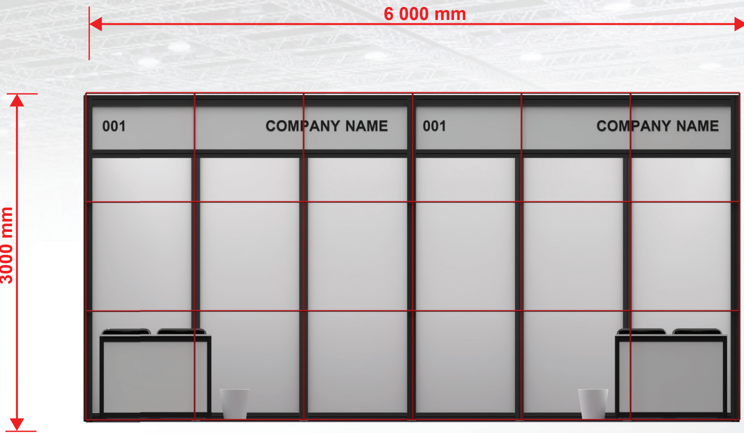
FRONT ELEVATION
